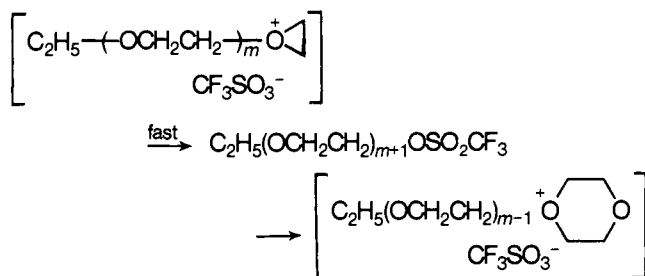
SCHEME X
