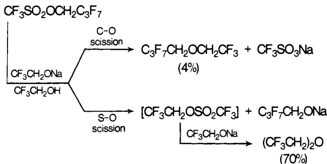
SCHEME IX
